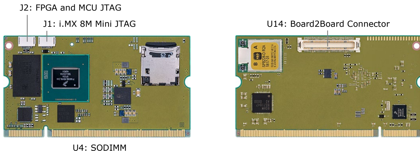
Figure 1-1: Connectors
