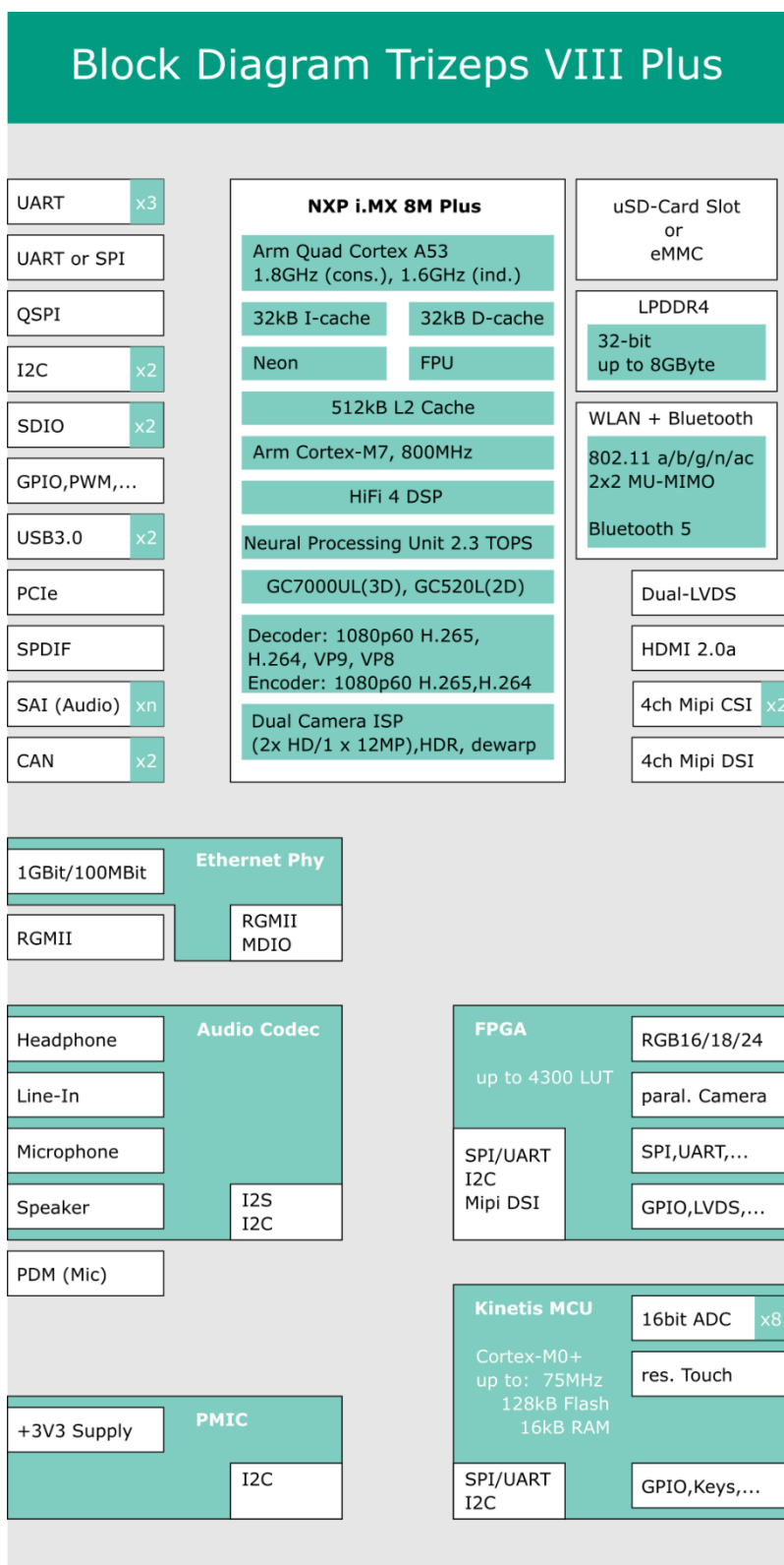
Figure 0-1: Simplified Block Diagram of Trizeps VIII Plus
