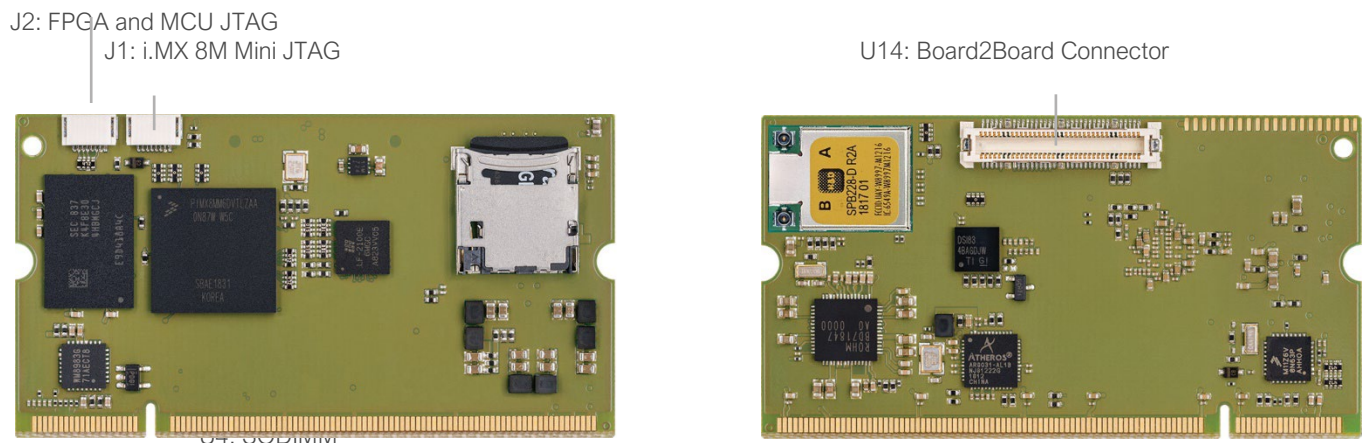
Figure 1-1: Connectors
